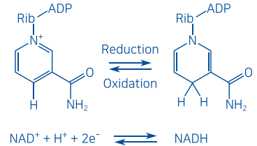
The redox reactions of nicotinamide adenine dinucleotide.
